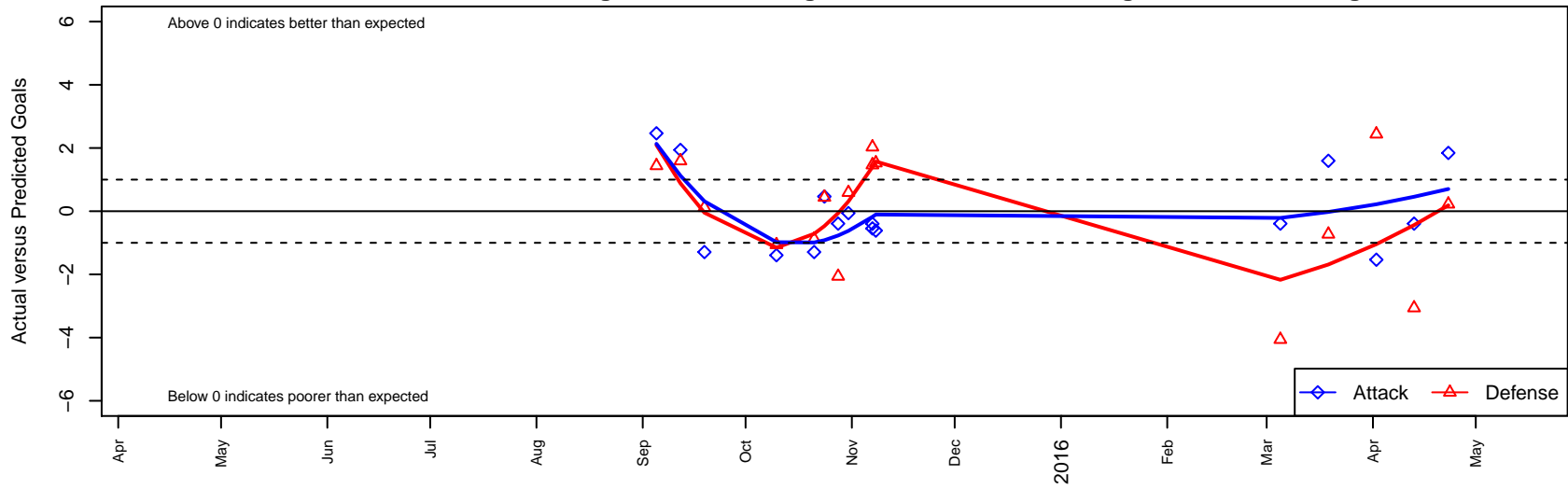
Idaho Rush White G04 Dots are actual minus expected GF (blue circles) and GA (red triangles). Blue line is smoothed change in attack strength. Red is smoothed change in defense strength.
